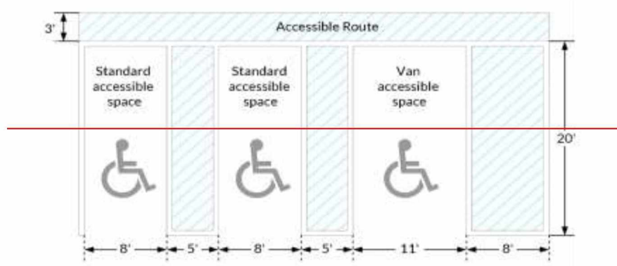
Figure 30.04-4: Accessible Space and Access Design
